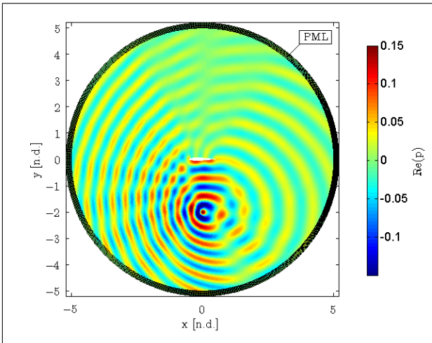
Figure 4. Contour plot: real part of the acoustic pressure. f=500 Hz, M_\infty = 0.3 and \alpha = 10^\circ .
