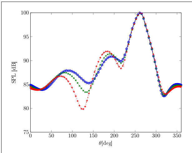
Figure 7. Sound pressure level. f = 100 \text{ Hz} , R_{fp} = 2.5L . \alpha = 10^\circ (solid - marker: +), \alpha = 4^\circ (dotted - marker: x) and \alpha = 0^\circ (dashed - marker: o). Scattering by a NACA 0012 from a monopole source with a non-uniform mean flow, dependency on the angle of attack.
