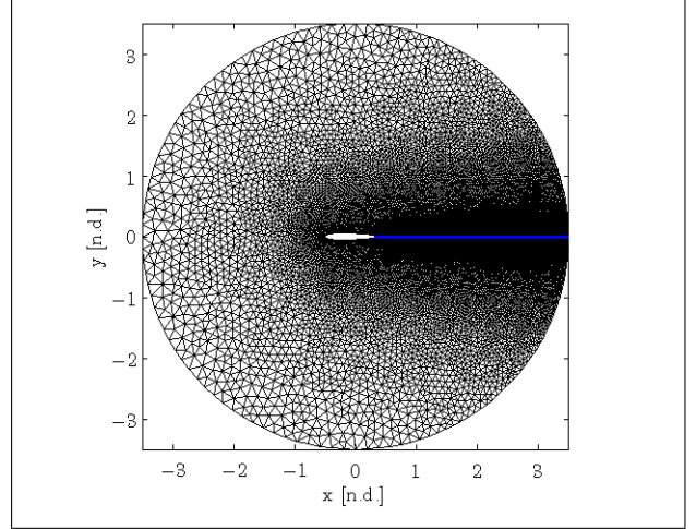
Figure 2. Aerodynamic mesh. Domain extent associated to \alpha = 6^\circ .
