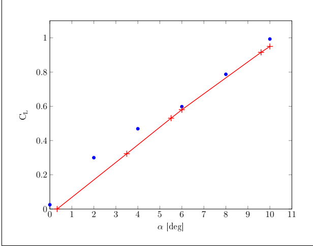
Figure 3. C_L as a function of the angle of attack. Validation against a viscous formulation. Eleni et al. [8] (solid); model proposed (dots).
